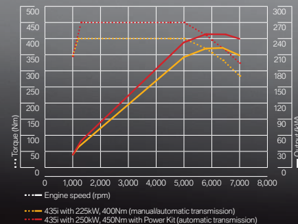
Performance data for the BMW 435i with BMW M Performance Power Kit Full load 435i
